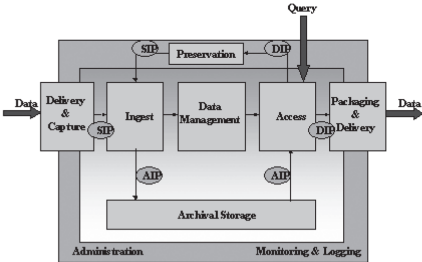
Figure 3. Model of the Open Archival Information System (OAIS)
